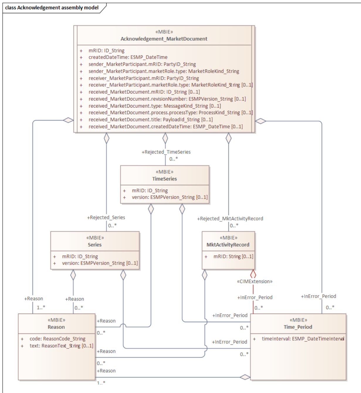
Figure 11 Class diagram: Ediel extended Acknowledgement Document assembly model
