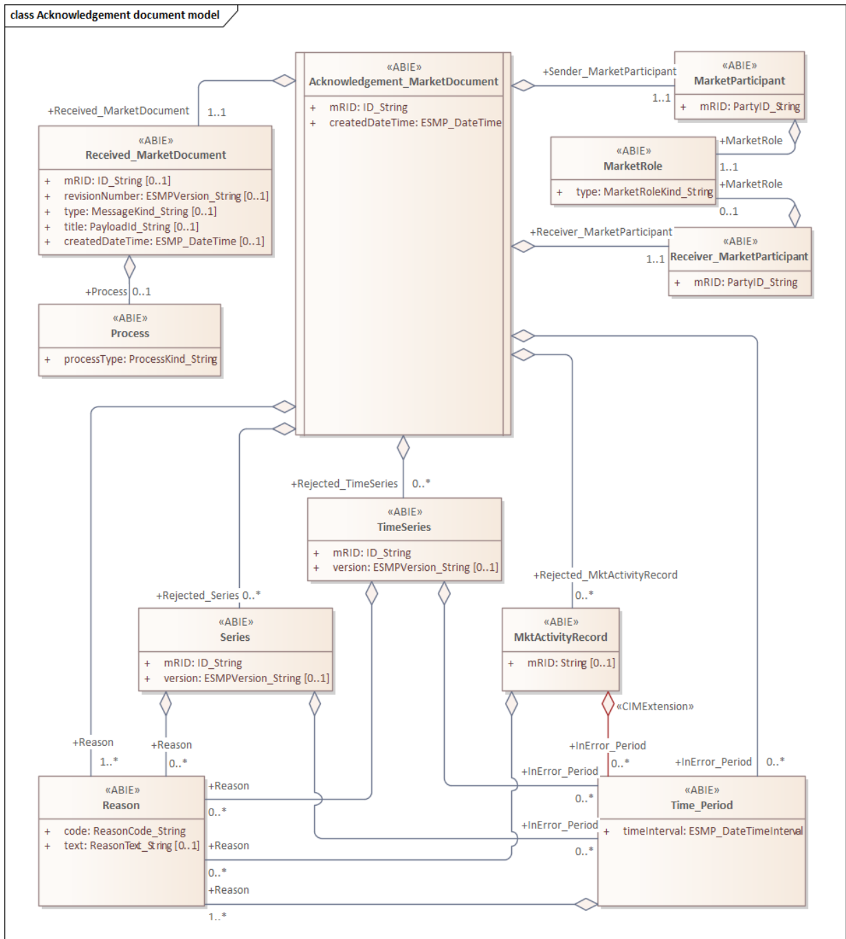
Figure 10 Class diagram: Ediel extended Acknowledgement Document contextual model
