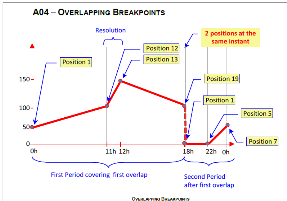
Figure 5: Curve type A04 Overlapping breakpoint
