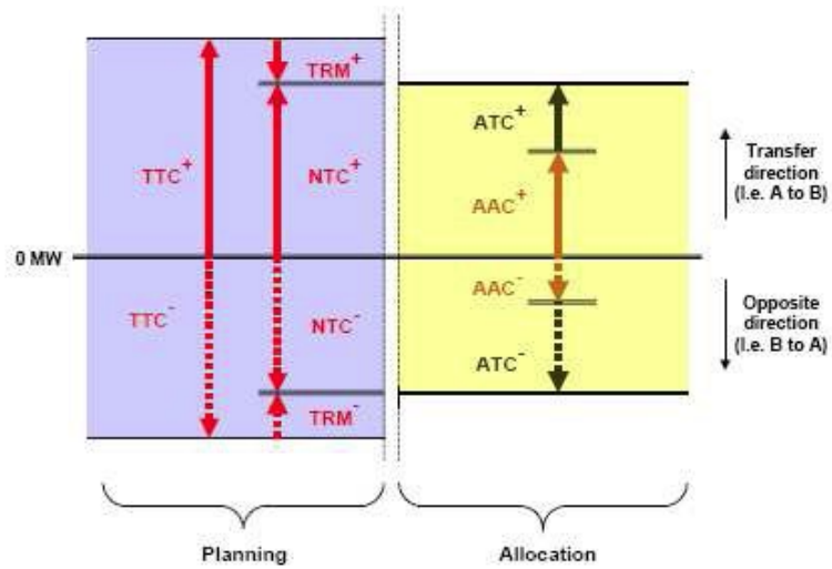
Figure 12: Transfer capacity definitions
