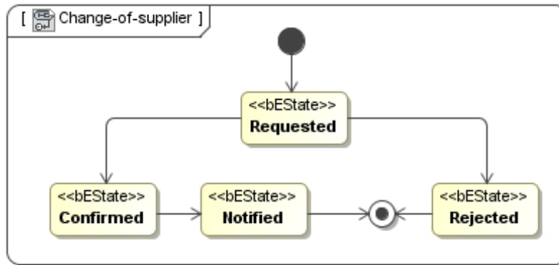
Figure 15 Business Entity State Diagram (example)
