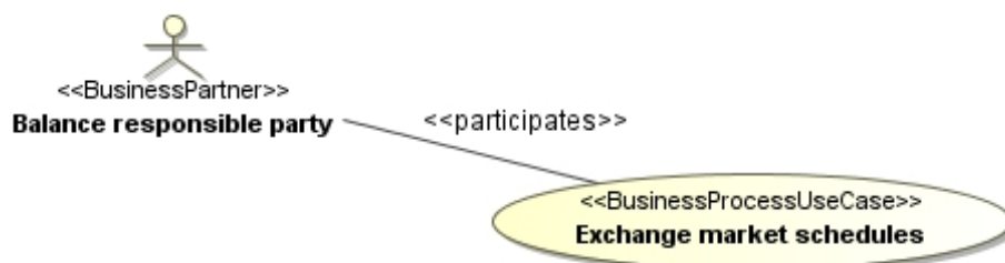
Figure 19 UseCase diagram, participate relationship
