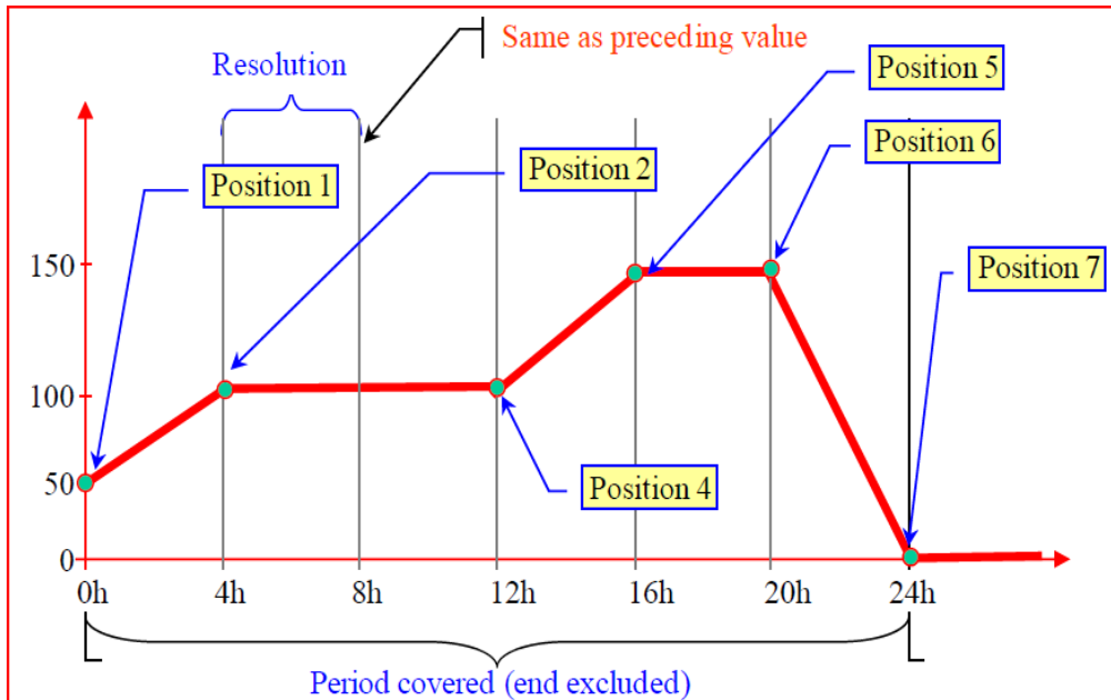
Figure 6: Curve type A05 Non-overlapping breakpoint
