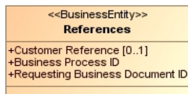
Figure 22 Class
