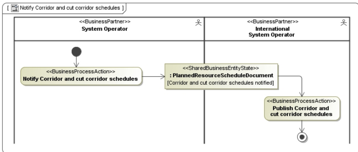
Figure 20 Activity diagrams
